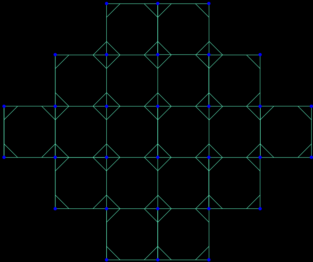
MODULAR ARRANGEMENT IN PLAN
